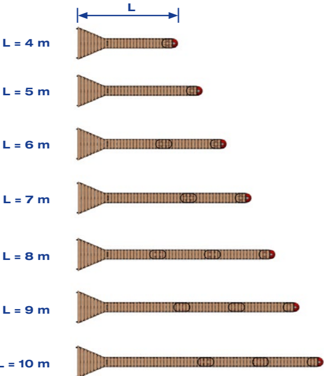
BOAT BOOMS WITH TIMBER DECKING
